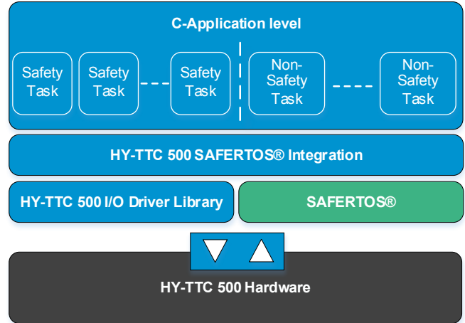
Figure: HY-TTC 500 SAFERTOS® integration diagram
